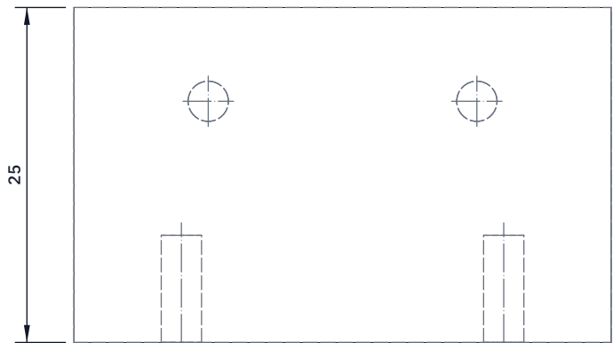
FRONT VIEW Scale 2:1; looking at the front (along +Y)
