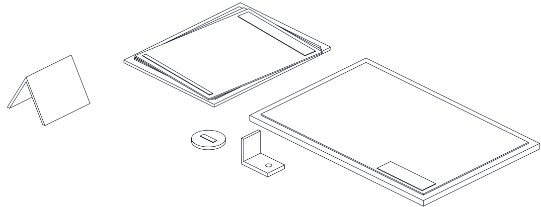
ISOMETRIC VIEW, ILLUSTRATIVE MASSING Not to scale; numbers match bom/bom.csv (see media/exploded.png)
