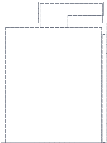
RIGHT VIEW Scale 1:25; looking at the right side (along -X)
