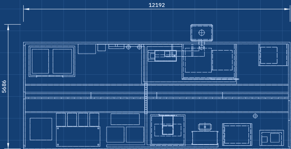
TOP VIEW Scale 1:100; looking down (along -Z)
