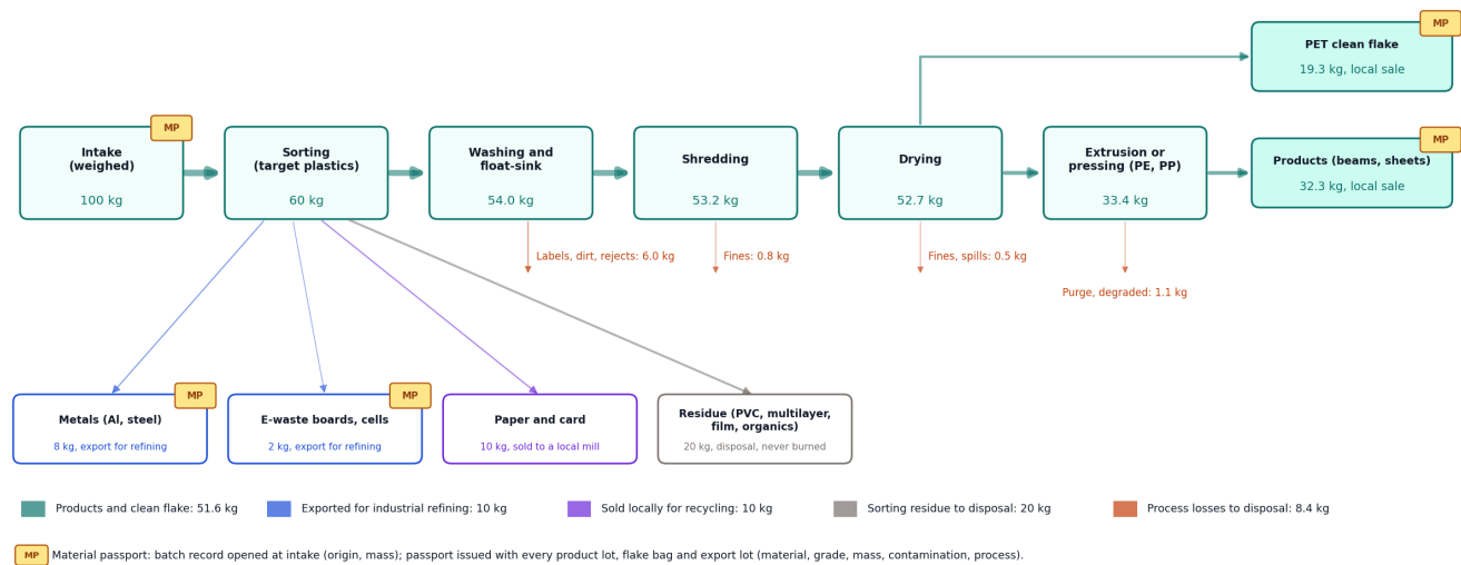
Figure 1. Material flow through the reference micro-factory per 100 kg of mixed collected input, from RFE-CAL-001. MP marks where a material passport record is opened (intake) and issued (every lot that leaves). All mass fractions are estimates.
