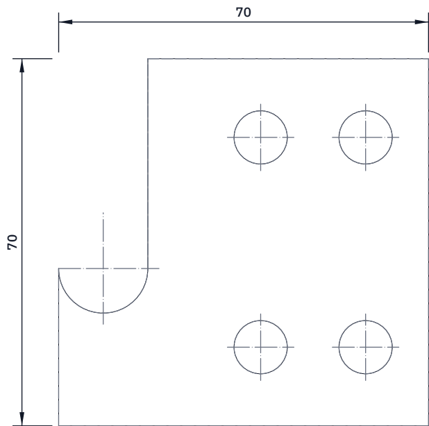
TOP VIEW Scale 1:1; looking down (along -Z)
