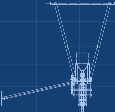
RIGHT VIEW Scale 1:20; looking at the right side (along -X)
