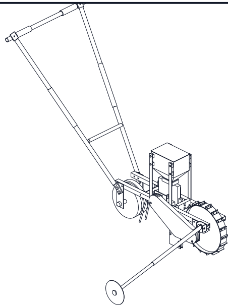
ISOMETRIC VIEW Not to scale; marker deployed; seen from the front right and above, about 30 deg elevation
