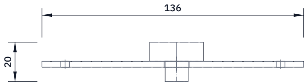
TOP VIEW Scale 1:2; looking down (along -Z)
