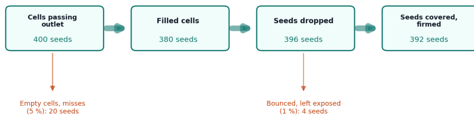
Figure 2. Seed flow over 100 m of row for the maize plate at 250 mm spacing. All values are estimates (the miss and double rates are assumptions carried into SDL-CAL-001); doubles add seeds, so more seeds are dropped than cells are filled.
