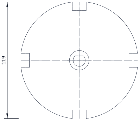
FRONT VIEW Scale 1:2; looking at the front (along +Y)
