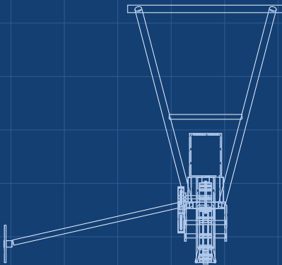
RIGHT VIEW Scale 1:20
