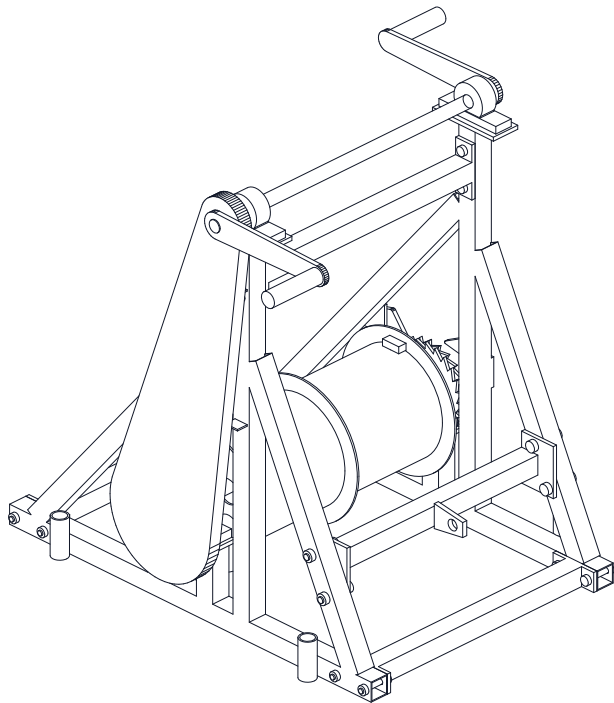
ISOMETRIC VIEW
