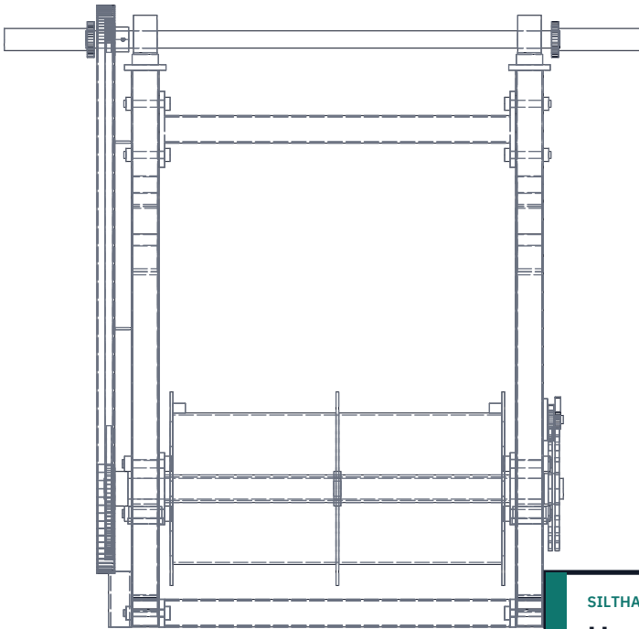
RIGHT VIEW
