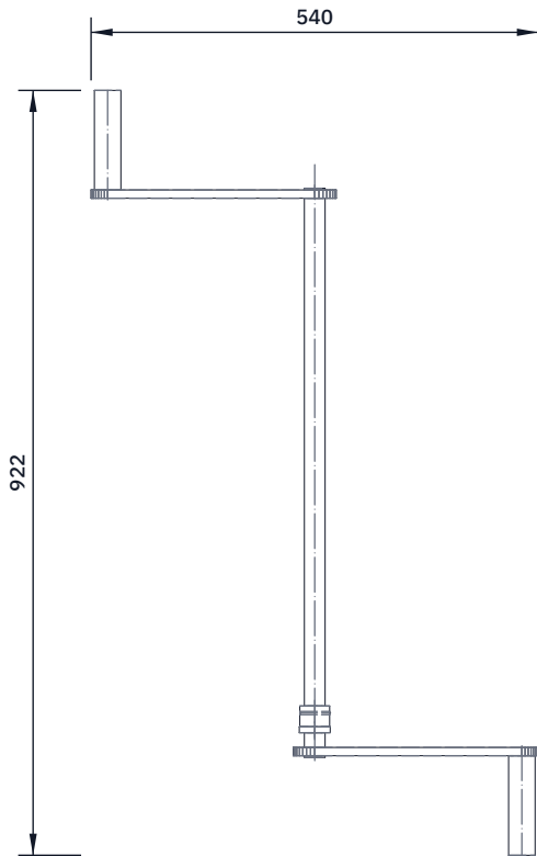
TOP VIEW
