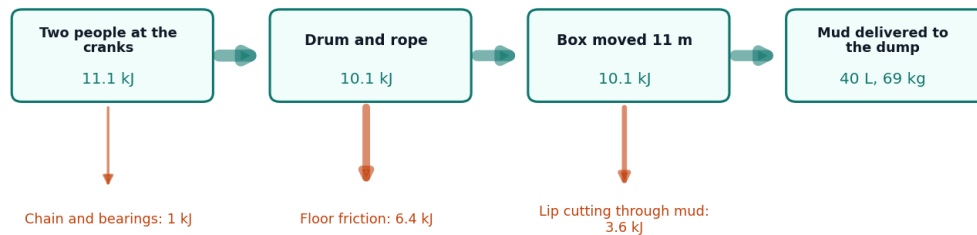
Figure 2. Energy for one 11 m haul of a full box (estimates): most of what the crank crew puts in goes to dragging the box over the floor.
