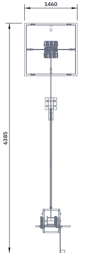
TOP VIEW
