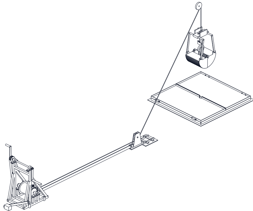
ISOMETRIC VIEW
