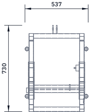
TOP VIEW Scale 1:20; looking down (along -Z)
