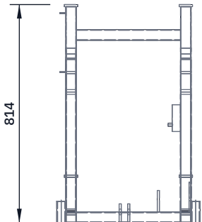
FRONT VIEW Scale 1:20; looking at the front (along +Y)
