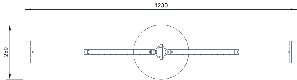
TOP VIEW Scale 1:10; looking down (along -Z)
