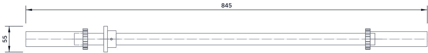
TOP VIEW Scale 1:5; looking down (along -Z)
