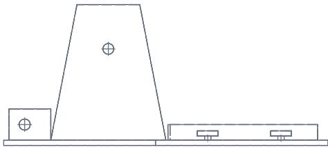
RIGHT VIEW Scale 1:10; looking at the right side (along -X)
