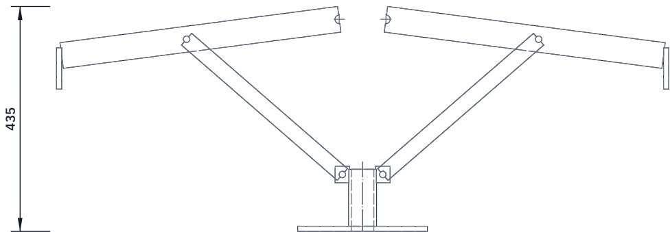
FRONT VIEW Scale 1:10; looking at the front (along +Y)
