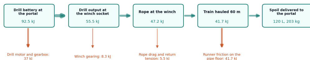
Figure 4. Energy per loaded 60 m haul (estimates): almost all of the work at the handle goes into dragging the sledges along the pipe floor.
