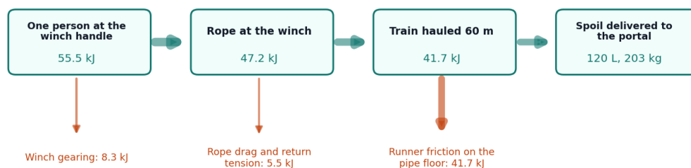
Figure 4. Energy per loaded 60 m haul (estimates): almost all of the work at the handle goes into dragging the sledges along the pipe floor.
