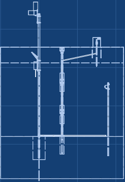
RIGHT VIEW Scale 1:100; looking at the right side (along -X)
