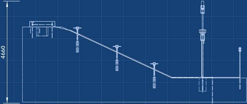
FRONT VIEW Scale 1:100; looking at the front (along +Y)
