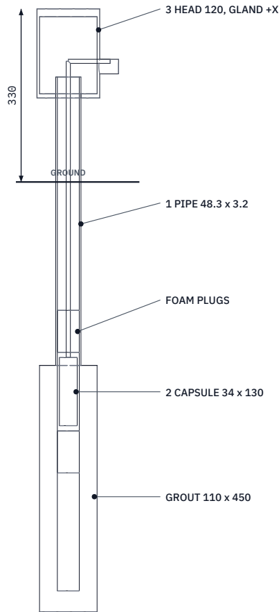
DETAIL A Stake section, scale 1:10
