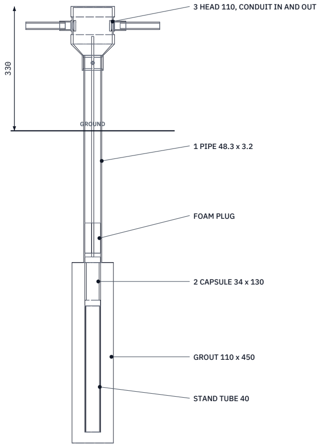
DETAIL A
