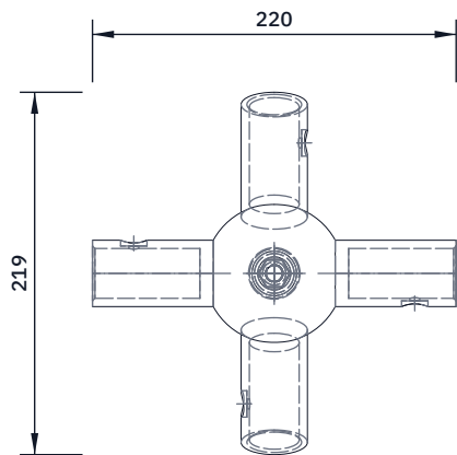
TOP VIEW Scale 1:5; looking down (along -Z)
