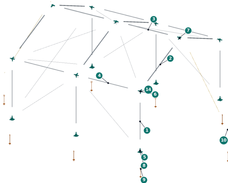
Figure 2. Exploded view with BOM numbers. The skin (item 11) is left out so the frame parts stay visible; items 12 and 13 are not modeled.
