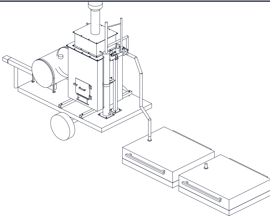
ISOMETRIC VIEW
