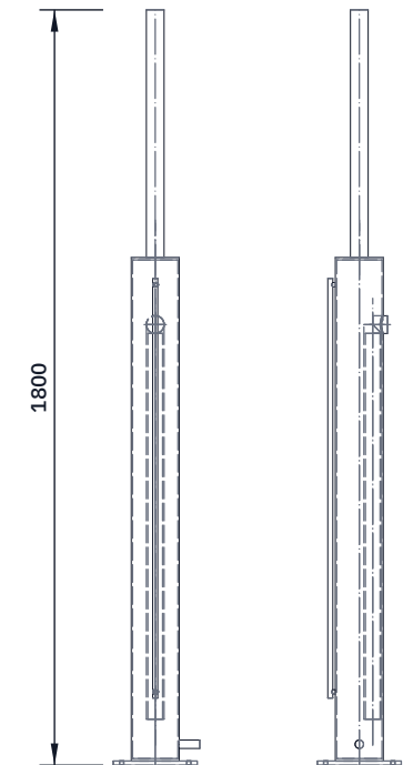
FRONT VIEW Scale 1:20; looking at the front (along +Y)
