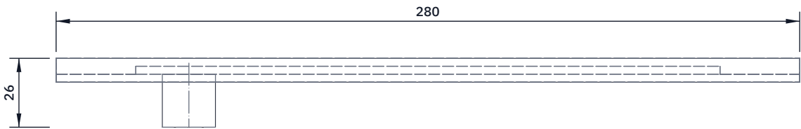
TOP VIEW Scale 1:2; looking down (along -Z)
