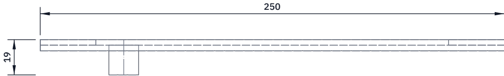
TOP VIEW Scale 1:2; looking down (along -Z)
