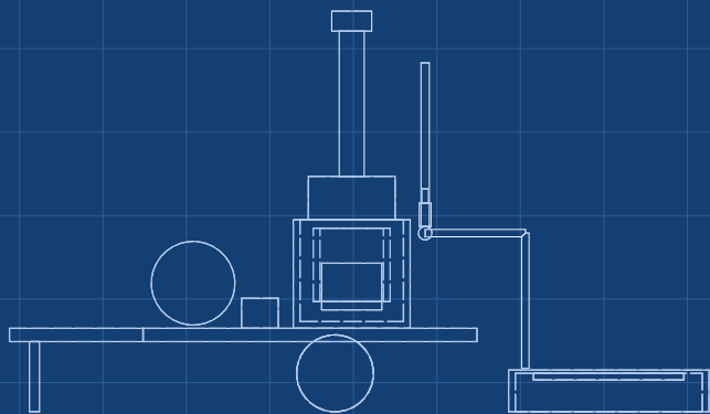
FRONT VIEW Scale 1:50
