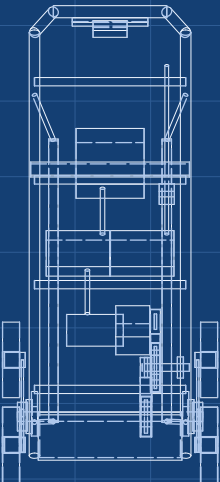
RIGHT VIEW Scale 1:20
