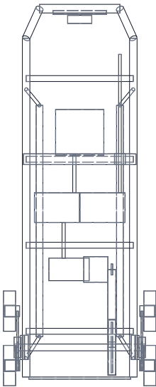
RIGHT VIEW Scale 1:20
