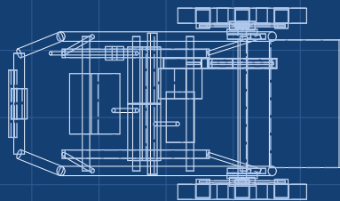
TOP VIEW Scale 1:20
