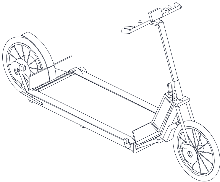
ISOMETRIC VIEW
