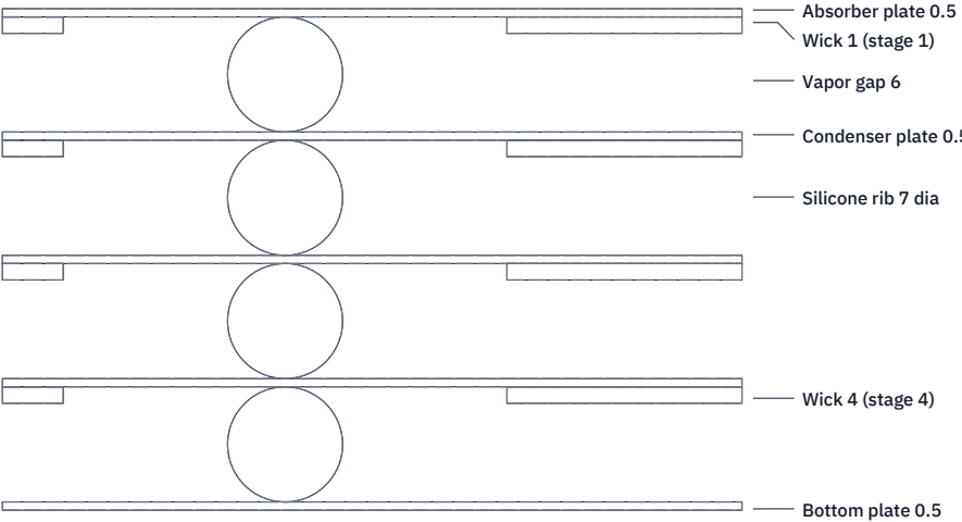
DETAIL A: STACK SECTION AT A RIB Scale 2:1, looking up the slope
