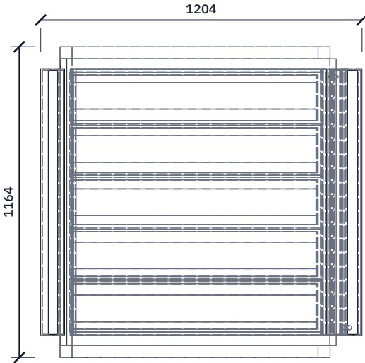
TOP VIEW Scale 1:20
