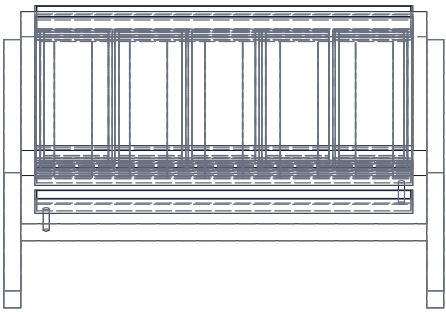
RIGHT VIEW (FROM LOW EDGE) Scale 1:20
