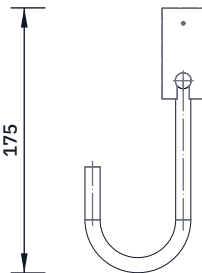
DETAIL B: HOOK HEAD
