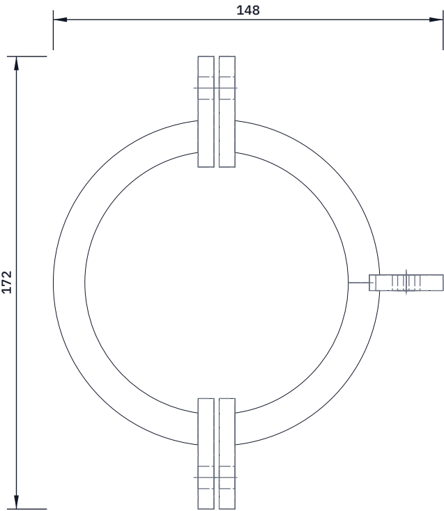
TOP VIEW Scale 1:2; looking down (along -Z)
