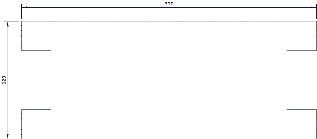
TOP VIEW Scale 1:2; looking down (along -Z)
