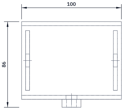
TOP VIEW Scale 1:2; looking down (along -Z)
