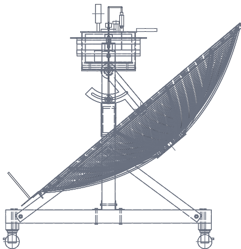
RIGHT VIEW
