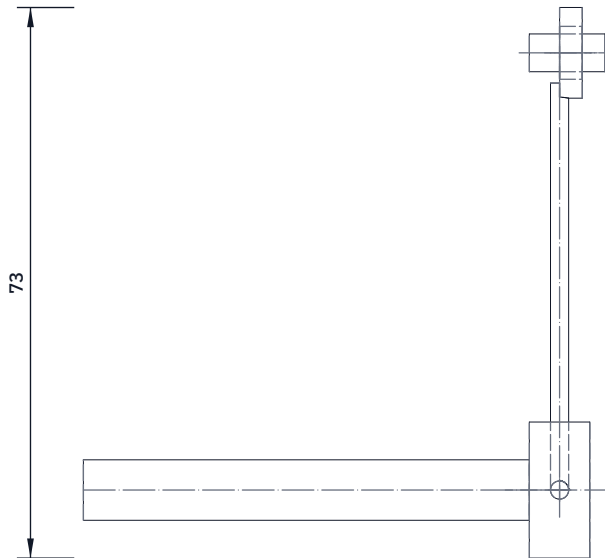
FRONT VIEW Scale 1:1; looking at the front (along +Y)
