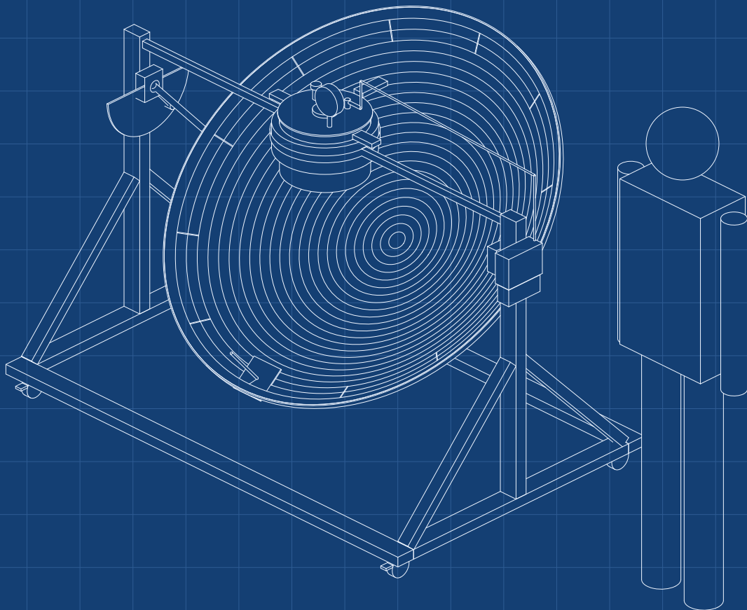
ISOMETRIC VIEW
