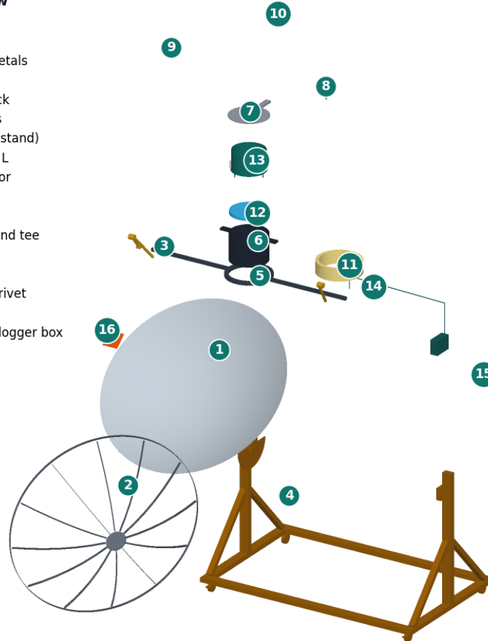
Figure 3. Exploded view with numbered callouts matching the BOM. The cooker parts are lifted out along the vertical axis. Items 17 to 21 are not modelled.
