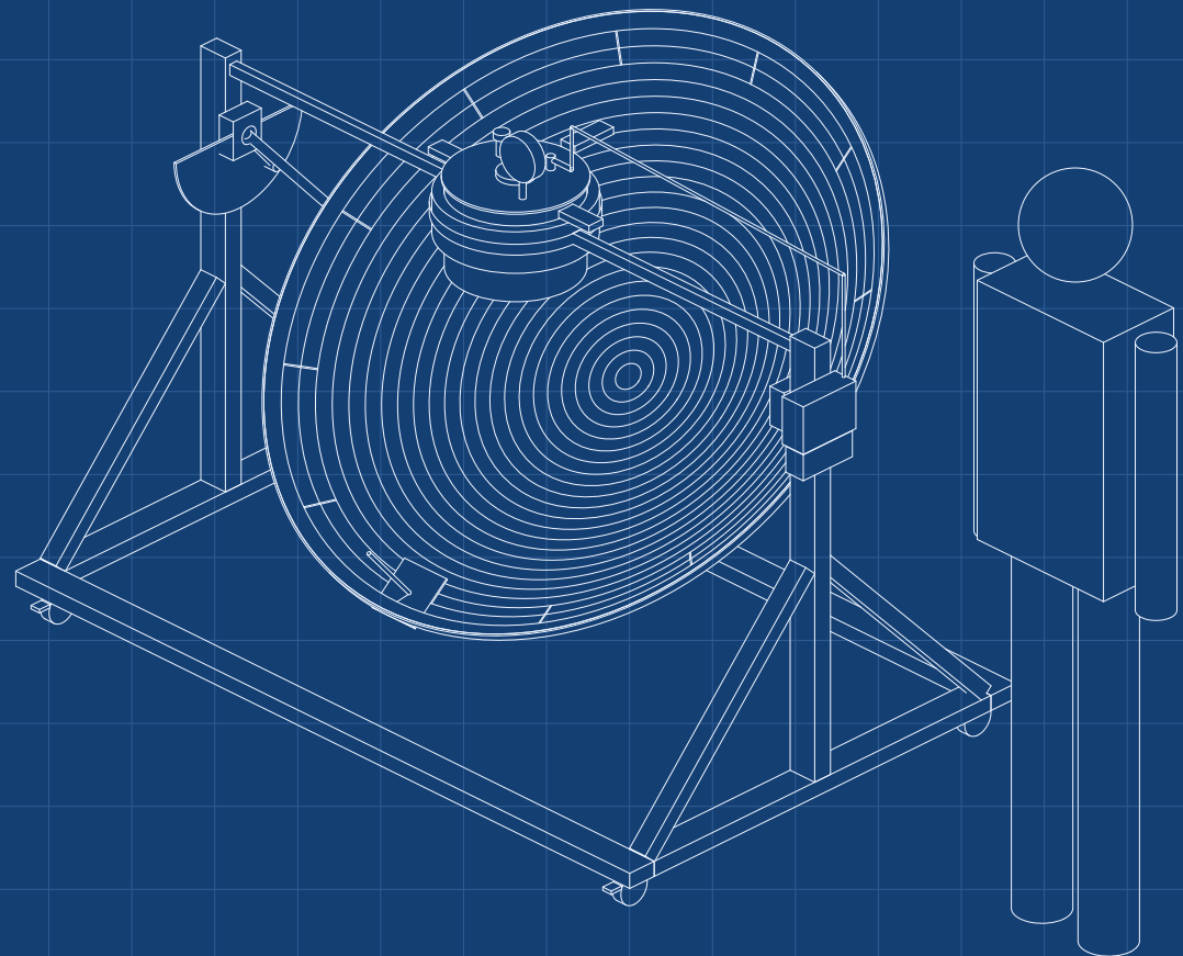
ISOMETRIC VIEW Not to scale; figure is a 1.75 m person
