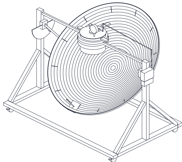
ISOMETRIC VIEW
