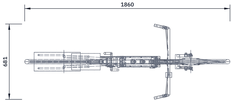
TOP VIEW Scale 1:20; looking down (along -Z)
