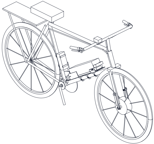
ISOMETRIC VIEW Not to scale; seen from the front right and above, about 30 deg elevation
