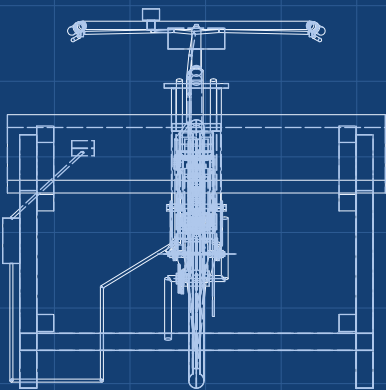
RIGHT VIEW Scale 1:20; looking at the right side (along -X)
