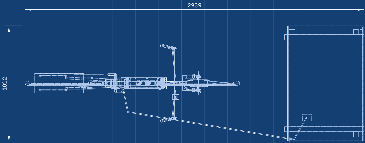
TOP VIEW Scale 1:20; looking down (along -Z)
